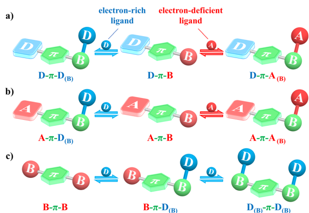
Fig. 24 The effect of coordination on the CT process of (a) D- \pi -B, (b) A- \pi -B and (c) B- \pi -B systems, D: electron-donor, A: electron-acceptor, and B: boron atom.
