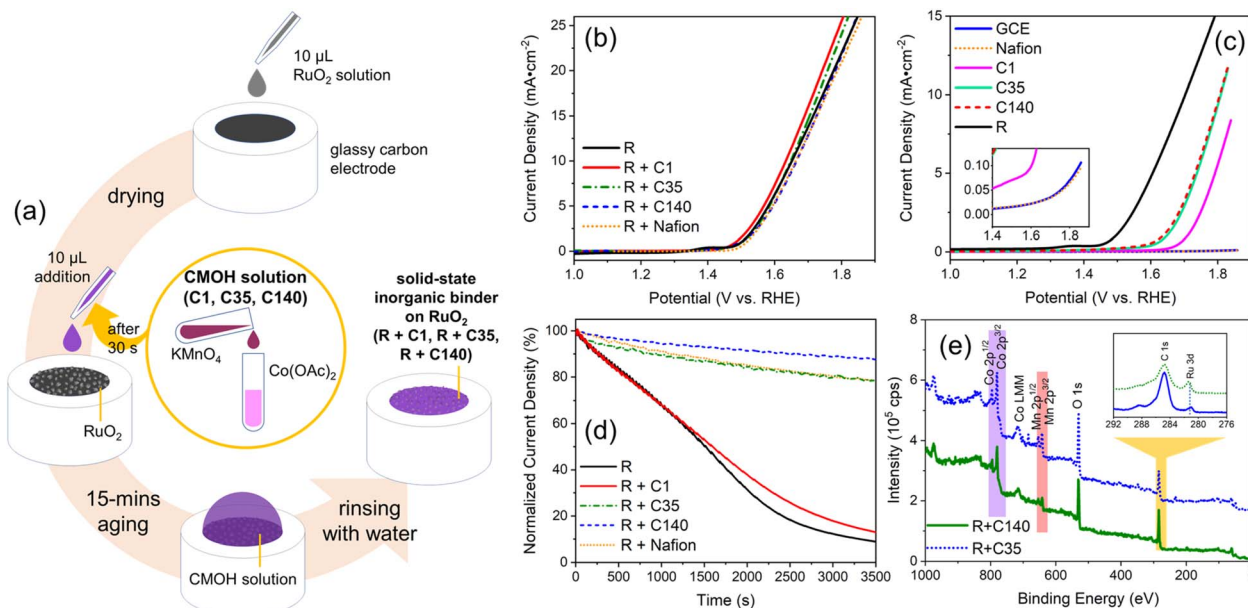
Fig. 1 Schematic illustration of the preparation of the \text{RuO}_2 catalyst immobilized by the inorganic solid-state binder CMOH on rotating-disc glassy-carbon electrodes (GCEs) (a) as well as various electrochemical tests and structural characterization studies of \text{RuO}_2 bound with different binders to GCE((b)–(d)) or \text{SiO}_2 wafers (e). (a) To bind the \text{RuO}_2 (denoted as R) drop-cast onto a glassy carbon electrode using CMOH, the binder is deposited onto the electrode surface through the aging of a mixed solution of \text{KMnO}_4 and \text{Co(OAc)}_2 (denoted as CMOH solution, yellow circle) with different concentrations (marked with labels C1, C35, and C140) at room temperature. (b) The linear scan voltammetry (LSV) curves showing the OER activities, under alkaline conditions, of \text{RuO}_2 immobilized by CMOH, prepared using CMOH solutions of varying concentrations. For comparison, the data for binder-free \text{RuO}_2 (R) and Nafion-bound \text{RuO}_2 (R + Nafion) are also shown. (c) The background LSV curves of the ( \text{RuO}_2 -free) Nafion- and CMOH-only samples. (d) The potentiostatic coulometry curves for the CMOH-bound \text{RuO}_2 samples recorded at 1700 rpm; the vertical axis shows the current densities normalized to the initial current density. The measurements are performed at a potential corresponding to 25 \text{ mA cm}^{-2} according to (b). (e) The survey XPS spectra of selected CMOH-bound \text{RuO}_2 samples over \text{SiO}_2 wafers; the inset shows the detailed comparison of C 1s and Ru 3d signals.
