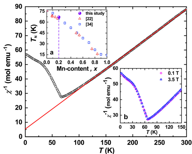
Fig. 4 Temperature dependence of reciprocal magnetic susceptibility for \text{Fe}_{0.8}\text{Mn}_{0.2}\text{WO}_4 ( \mu_0H = 3.5 T) together with the Curie–Weiss fit (red line). Inset a: dependence of critical Néel-temperatures ( T_N ) versus Mn content ( x ) in \text{Fe}_{1-x}\text{Mn}_x\text{WO}_4 . Inset b: temperature dependence of reciprocal magnetic susceptibility for \text{Fe}_{0.8}\text{Mn}_{0.2}\text{WO}_4 in different magnetic fields.
