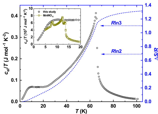
Fig. 6 Temperature dependence of the electronic specific heat of \text{Fe}_{0.8}\text{Mn}_{0.2}\text{WO}_4 in the c_{\text{el}}/T(T) presentation (left black scale) together with the temperature evolution of the magnetic entropy near an antiferromagnetic transition. Inset: low-temperature dependencies of c_{\text{el}}/T(T) for \text{Fe}_{0.8}\text{Mn}_{0.2}\text{WO}_4 together with the literature data for \text{MnWO}_4 . 37 The latter were divided by 20 for better visualization.
