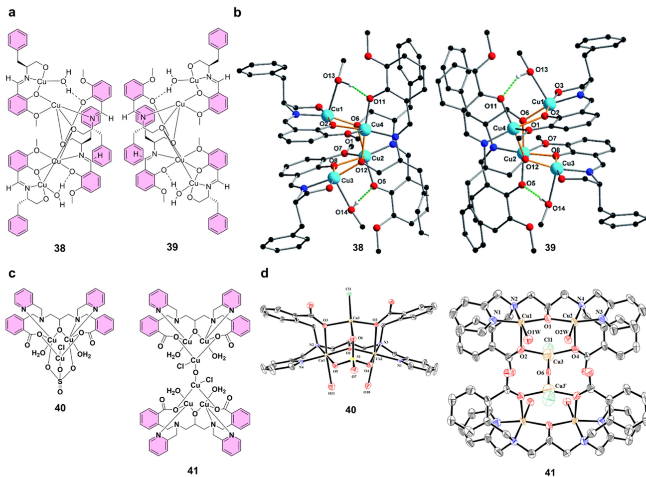
Fig. 4 (a) Structures of complexes 38 and 39. (b) Molecular representations of complexes 38 and 39, with hydrogen atoms and nitrate counterions omitted for clarity. Hydrogen bonds are indicated by green dashed lines. Atom color scheme: Cu (light blue), N (blue), O (red), and C (black). Reproduced from ref. 4f with permission from the Royal Society of Chemistry, copyright 2019. (c) Structures of complexes 40 and 41. (d) ORTEP representations of the X-ray crystal structures of complexes 40 and 41, shown with 35% probability ellipsoids. For complex 40, all hydrogen atoms and crystallized water molecules are omitted for clarity. For complex 41, hydrogen atoms and counteranions are omitted. Color codes: Cu (brown), N (blue), O (red), S (yellow), Cl (light green), and C (black). Reproduced from ref. 17 with permission from the American Chemical Society, copyright 2024.
