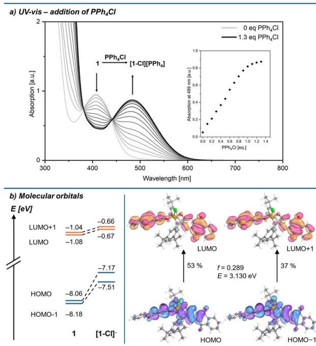
Fig. 4 (a) Change in the experimental UV-vis absorption spectrum of 1 ( 5.84 \times 10^{-4} M in DCM) upon stepwise addition of PPh 4 Cl ( K_C \approx 3.6 \times 10^5 mol −1 l). (b) Energy change in the frontier molecular orbitals upon chloride coordination in 1 and orbital transitions contributing to the low-energy CT excitation in the chloride adduct ( f = oscillator strength; E = transition energy; transition energy given without 0.56 eV redshift; ωB97X-D3/def2-TZVPP/SMD(DCM)// r^2 SCAN-3c).
