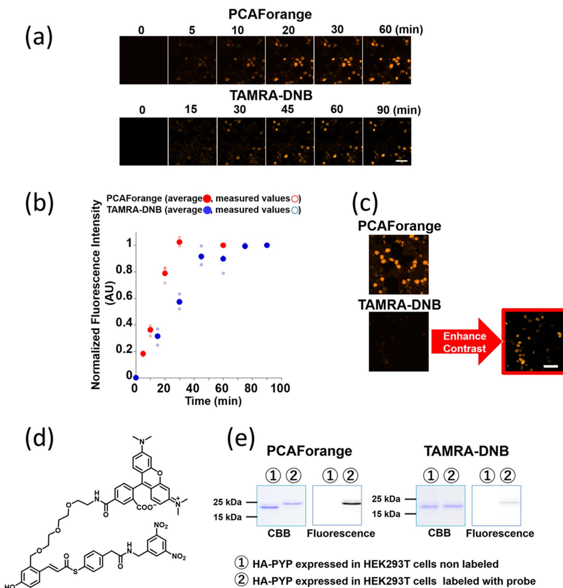
Fig. 4 Comparison of the labeling performance of PCAForange against TAMRA-DNB. (a) Time-lapse imaging of PYP-NLS expressed in HEK293T cells labeled with 1 \mu M PCAForange or 1 \mu M TAMRA-DNB. Scale bar: 50 \mu m. (b) Quantification of the fluorescence intensity of PYP-NLS labeled with PCAForange (red solid circles) and TAMRA-DNB (blue solid circles). Data points plotted are means of the mean of triplicate measurements (open circles) with error bars representing the standard deviations. (c) Comparison of the brightness of PCAForange- and TAMRA-DNB-labeled PYP-NLS in HEK293T cells imaged at the same laser intensity. Due to low signal intensity, TAMRA-DNB-labeled cells could only be visualized with contrast enhancement. Scale bar: 50 \mu m. (d) Chemical structure of TAMRA-DNB. (e) SDS-PAGE analysis of labeling efficiency of PCAForange and TAMRA-DNB in live HEK293T cells.
