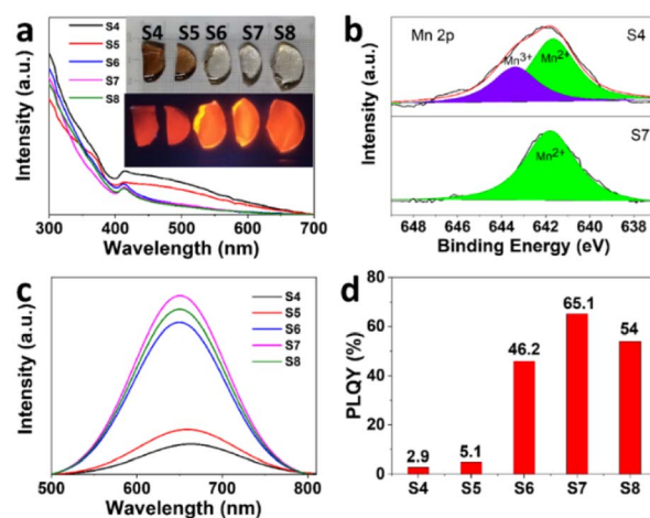
Fig. 3 The influence of the amount of Cs 2 CO 3 on the final product of the CsMnBr 3 NC embedded glasses. (a) UV-vis absorption spectra. Inset shows photographs of a series of CsMnBr 3 NC embedded glasses under daylight and UV light. (b) Mn 2p XPS spectra of samples S4 and S7. (c) PL emission spectra and (d) the PLQY of a series of CsMnBr 3 NC embedded glasses with different amounts of Cs 2 CO 3 . Note: 15SiO 2 –30B 2 O 3 –10ZnO–xCs 2 CO 3 –1MnCO 3 –10NaBr (x = 1, 1.5, 1.75, 2, and 2.25, denoted as S4, S5, S6, S7, and S8).
