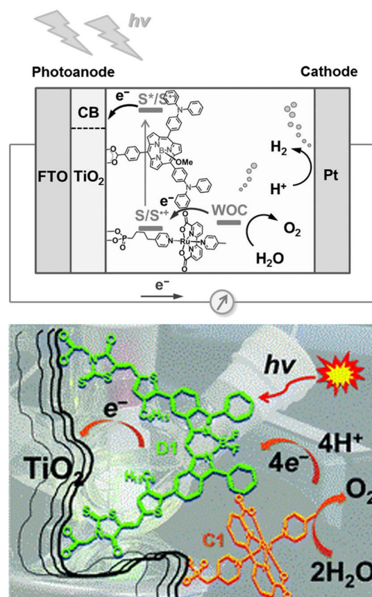
Fig. 14 Photosynthetic systems combining a Ru(bda) WOC and a subporphyrin (top) or BODIPY (bottom) photosensitizer, anchored onto a \text{TiO}_2 semiconductor. Reprinted from ref. 105 and 106 with permission from the Royal Society of Chemistry, copyright 2016 and 2017.
