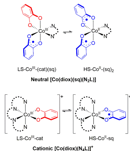
Fig. 1 Valence tautomeric interconversions for [\text{Co}(\text{diox})(\text{sq})(\text{N}_2\text{L})] and [\text{Co}(\text{diox})(\text{N}_4\text{L})]^+ families of Co–dioxolene complexes.
