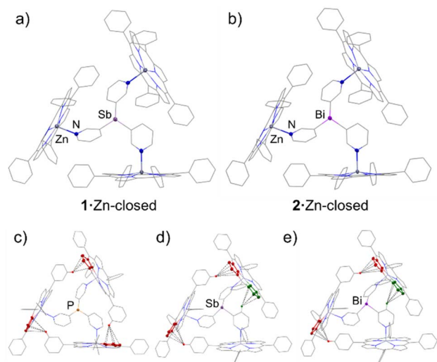
Fig. 4 X-ray structures of the complexes 1 ·Zn-closed (a) and 2 ·Zn-closed (b). In both structures, the ligand coordinates three porphyrins, leading to the formation of capsule-type structures. Solvent molecules and H-atoms are omitted for clarity. Selected bond lengths (Å) and angles (°): 1 ·Zn, Sb–C py range 2.146(5)–2.158(5); N py –Zn range 2.149(4)–2.194(4); C py –Sb–C py range 95.4(2)–96.0(2). 2 ·Zn, Bi–C py range 2.235(6)–2.261(5); N py –Zn range 2.149(5)–2.184(5); C py –Bi–C py range 93.0(2)–94.2(2). Colour key: C (grey), Zn (dark grey), N (blue), P (orange), Sb (light purple), Bi (purple). X-ray structures of [\text{P}(3\text{-py})_3] \cdot (\text{ZnTPP})_3 (c), 1 ·Zn (d) and 2 ·Zn (e) showing the capsules with close intramolecular CH– \pi interactions between ZnTPP building blocks highlighted in red and interactions between C–H pyridyl and ZnTPP highlighted in green. CH– \pi interaction lengths (Å): [\text{P}(3\text{-py})_3] \cdot (\text{ZnTPP})_3 2.725, 2.893 and 2.960; 34 1 ·Zn 2.971, 3.051 and 2.978 (CH py – \pi ); 2 ·Zn 2.991, 3.025 and 2.978 (CH py – \pi ).
