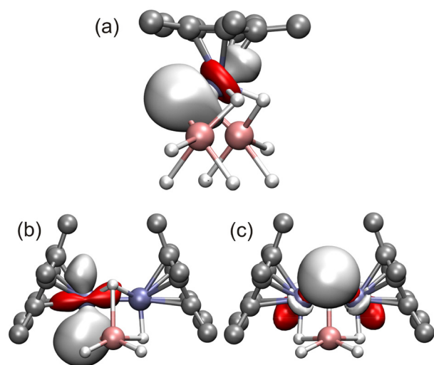
Fig. 9 Cr–H bonding NBOs in complex 10 : (a) one of the four Cr–H bonds of the mononuclear unit, (b) one of the two Cr–H bonds of the dinuclear unit, and (c) bridging Cr 2 –H bond of the dinuclear unit. Color code: C = gray, H = white, Cr = iceblue, Al = pink. Hydrogen atoms of the \eta^5 -C 5 Me 5 ligands are omitted for clarity.
