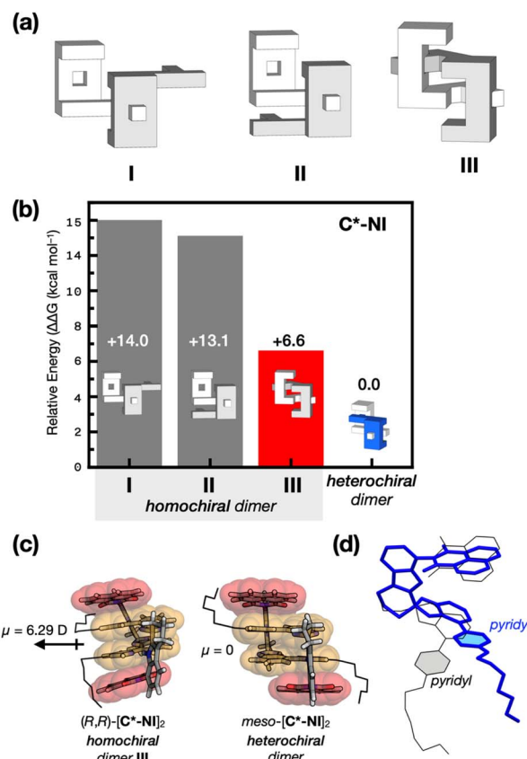
Fig. 5 (a) Schematic representations of possible structures of the homochiral dimer (R,R)\text{-}[\text{C}^*\text{-NI}]_2 . (b) Bar graphs comparing the free energies computed at the B3LYP-D3/6-31++G** level, relative to the energy of the heterochiral dimer as the reference point. (c) Dipole moments of energy-minimized DFT models of the homochiral (R,R)\text{-}[\text{C}^*\text{-NI}]_2 ( III in (a)) and meso - [\text{C}^*\text{-NI}]_2 . (d) Overlaid DFT energy-minimized structures of \text{C}^*\text{-NI} comprising the homochiral (blue capped-stick) vs. heterochiral (black wireframe) dimer.
