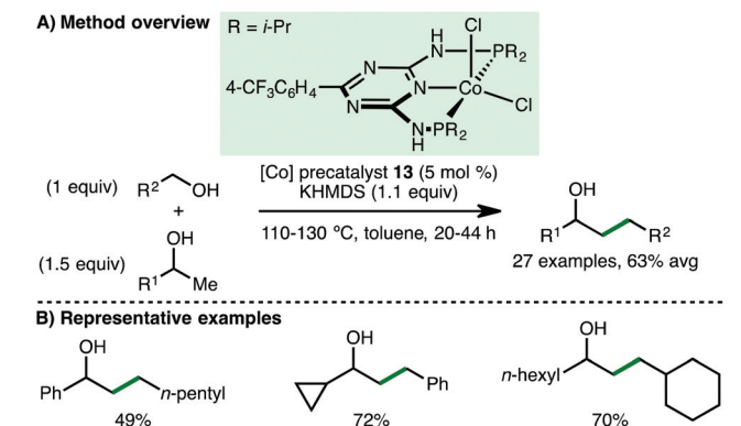
Scheme 21 Co-Catalysed cross coupling of 2° and 1° alcohols (Kempe).
