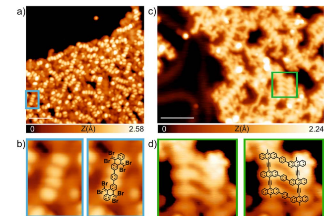
Fig. 8 On-surface deposition and reactivity of TBQ3 species on Au(111). (a) Overview STM image of the sublimation of a submonolayer coverage of TBQ3 on a pristine Au(111) surface kept at room temperature. V_b = 1 V, I_t = 100 pA, scale bar: 4.0 nm. (b) Left: Zoomed-in image of the blue rectangle indicated in panel (a) showing an intact molecule with two consecutive pairs of elongated bright protrusions. Right: Superposition of the chemical model. (c) Long-range STM image after the annealing of (a) at 150 °C. V_b = 0.5 V, I_t = 50 pA, scale bar: 4 nm. (d) Left: Zoomed-in image of the green highlighted area in panel (c). Right: Superposition of the chemical model.
