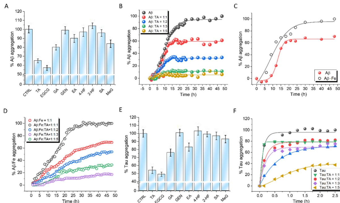
Fig. 3 Screening of PPs for their ability to inhibit A\beta_{42} and tau aggregation monitored using ThT assay ( \lambda_{\text{ex}} = 444 nm and \lambda_{\text{em}} = 484 nm). [ A\beta_{42} ] = 10 \mu\text{M} , [Tau] = 5 \mu\text{M} . (A) Effect of PP on A\beta_{42} aggregation. [PP] = 20 \mu\text{M} . (B) Kinetics of A\beta_{42} aggregation in the presence of increasing concentrations of TA (10 to 50 \mu\text{M} ). (C) Comparison of kinetic curves of A\beta_{42} aggregation and Fe-induced A\beta_{42} aggregation. [ \text{FeCl}_3 ] = 10 \mu\text{M} . (D) Kinetics of Fe-induced A\beta_{42} aggregation in the presence of an increasing concentration of TA (10 to 50 \mu\text{M} ). (E) Screening of PPs for their ability to inhibit AA-induced tau aggregation. [PP] = 20 \mu\text{M} , and [AA] = 185 \mu\text{M} . (F) Kinetics of tau aggregation in the presence of increasing concentrations of TA (5 to 25 \mu\text{M} ). AA: arachidonic acid.
