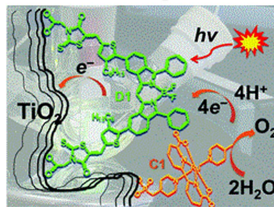
Fig. 14 Photosynthetic systems combining a Ru(bda) WOC and a subporphyrin (top) or BODIPY (bottom) photosensitizer, anchored onto a \text{TiO}_2 semiconductor. Reprinted from ref. 105 and 106 with permission from the Royal Society of Chemistry, copyright 2016 and 2017.
