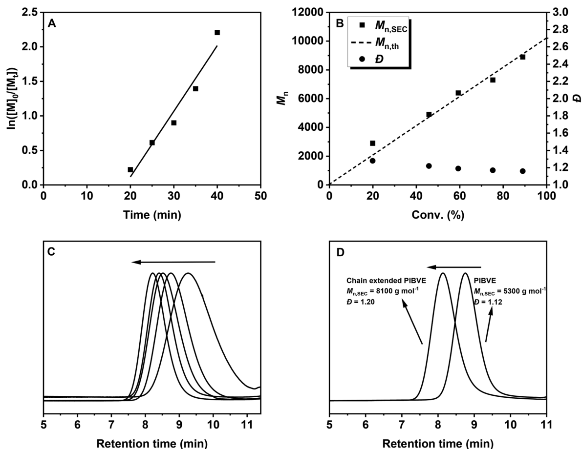
Fig. 2 Polymerization of IBVE with [IBVE] 0 /[DTCEB] 0 /[DPI] 0 /[Ir(ppy) 3 ] 0 = 100/1/0.01/0.0001 under a 450 nm blue LED at −30 °C in toluene and DCM (v/v = 9 : 1), V IBVE = 1 mL, V solvent = 1 mL. (A) ln([M] 0 /[M] t ) versus time. (B) Molecular weight ( M n ) and molecular weight distribution ( Đ ) versus monomer conversion; (C) SEC traces of the obtained PIBVE; (D) SEC traces of the PIBVE before and after chain extension.
