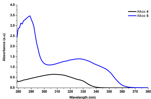
Fig. 1 UV – Visible spectra overlay of bromo tacrine-based alkoxyamine 4 and D- \pi -A tacrine TMIO-based alkoxyamines 5 in tert -butyl benzene with concentration = 1.0 \times 10^{-4} M.
