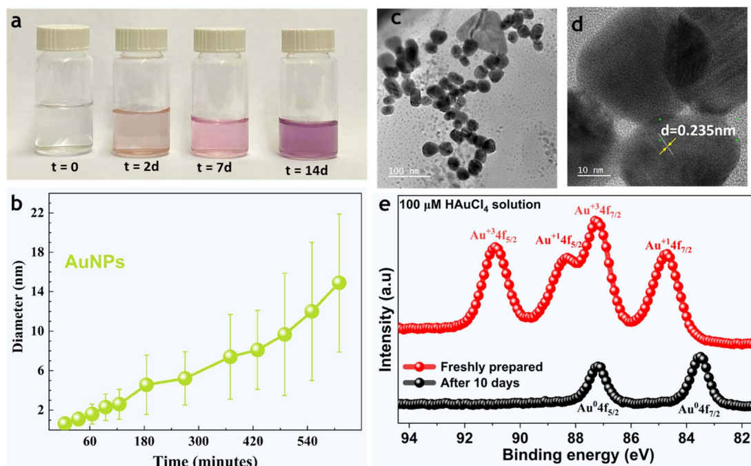
Fig. 2 Spontaneous formation and growth of AuNPs in bulk 100 μM HAuCl 4 in water. (a) Bulk solution changing color due to the nucleation and growth of AuNPs. (b) Formation and growth of particles with time, as measured by DLS. (c) TEM micrograph showing the presence of AuNPs of different sizes. (d) TEM imaging showing an interlayer spacing of ~0.235 nm corresponding to the Au(111) atomic plane of metallic gold Au(0). (e) XPS analysis showing the presence of Au 3+ and Au + in the freshly prepared solution and Au(0) in the 10-days-old solution, revealing the complete reduction of gold ions to AuNPs after some time.
