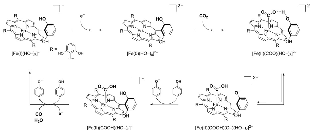
Scheme 4 The proposed CO 2 -to-CO electroreduction mechanism by iron porphyrin catalyst Fe2.
