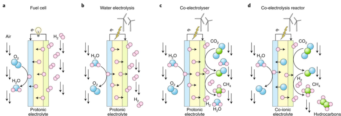
Fig. 15 The different working principles of H-SEMRs: (a) fuel cell, (b) electrolyzer cell, (c) \text{CO}_2/\text{H}_2\text{O} co-electrolysis, and (d) co-electrolysis reactor based on co-ionic conductor. 66,265 Reproduced with permission.
