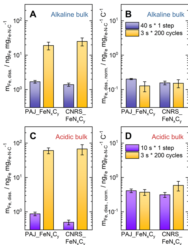
Fig. 6 The Fe dissolution data of PAJ_ \text{FeN}_x\text{C}_y and CNRS_ \text{FeN}_x\text{C}_y during the 200-cycle AST (each cycle: 3 s at j^* \text{mA cm}^{-2} and 3 s at -0.1 \text{ mA cm}^{-2} , yellow bars) and the t -s galvanostatic step at j^* \text{mA cm}^{-2} . The duration t of the galvanostatic step is 40 s in alkaline media (A & B, indigo bars) or 10 s in acidic media (C & D, violet bars), and the current density j^* is -75 \text{ mA cm}^{-2} for CNRS_ \text{FeN}_x\text{C}_y in Acidic-HT, and -100 \text{ mA cm}^{-2} for all the others (see Table 1). The amount of the dissolved Fe species has been normalized to the catalyst loading (A & C) or both the catalyst loading and the ORR charge (B & D). The error bars are equal to the differences between the results of the two measurements.
