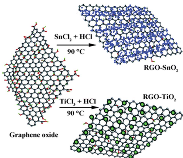
Fig. 4 One-pot synthesis of \text{SnO}_2/\text{graphene} and \text{TiO}_2/\text{graphene} photocatalysts. Reprinted from ref. 59.
