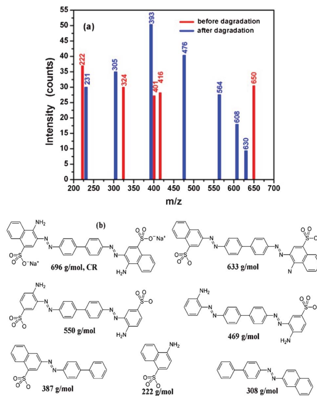
Fig. 10 Spectra of CRS before and after degradation (a) and the CR and possible degradation products of CR (b).
