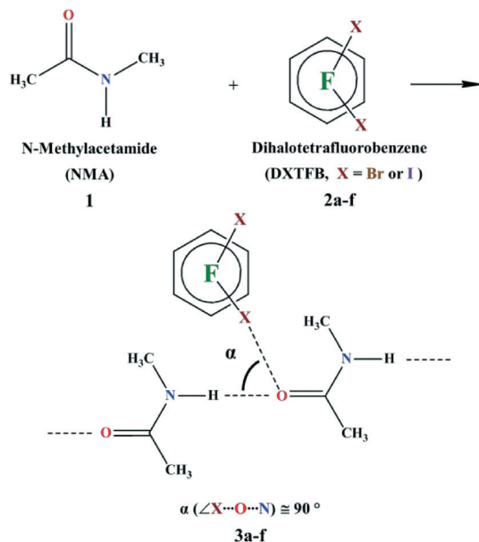
Scheme 1 Synthesis of N -methylacetamide (NMA, 1 ) co-crystals with various dihalotetrafluorobenzenes (DXTFB, X = Br or I). The orthogonal angle ( \alpha ) is defined as the angle between XB ( C-X \cdots O , X = Br or I) and HB ( N-H \cdots O ), i.e., \angle X \cdots O \cdots N .
