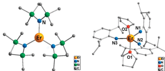
Fig. 6 Molecular structures of the complexes [\text{Er}\{\text{N}(\text{SiMe}_3)_2\}_3] (left) and [\text{Er}\{\text{NHPh}^1\text{Pr}_2\}_3(\text{THF})_2] (right), with hydrogen atoms omitted for clarity. Adapted with permission from ref. 22. Copyright 2014 American Chemical Society.
