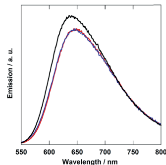
Fig. 3 The emission spectra of Ru (CH 2 OCH 2 ) Re (red), Ru (CH 2 SCH 2 ) Re (blue), and Ru (CH 2 CH 2 CH 2 ) Re (black) collected at 25 °C in DMF; the spectra are normalized to the absorbance of the solutions at \lambda_{\text{excitation}} = 456 nm.
