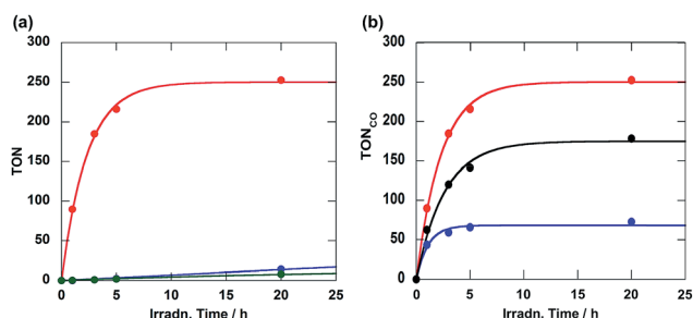
Fig. 2 (a) Turnover number of Ru (CH 2 OCH 2 ) Re for CO (red), HCOOH (green), and H 2 (blue) formation and (b) those of Ru (CH 2 OCH 2 ) Re (red), Ru (CH 2 SCH 2 ) Re (black), and Ru (CH 2 CH 2 CH 2 ) Re (blue) for CO formation as a function of irradiation time. DMF–TEOA (5 : 1) solutions containing 0.05 mM of the diad and 0.1 M of BNAH were irradiated at \lambda > 500 nm under a CO 2 atmosphere.
