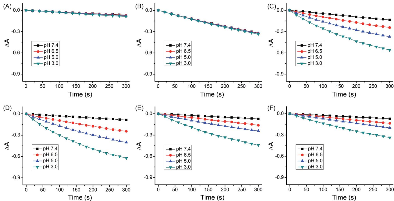
Fig. 4 Rate of decay of ABDA sensitized by (A) control, (B) [Ru(bpy)_3]Cl_2 , (C) 1 , (D) 2 , (E) 3 and (F) 4 in aerated disodium hydrogen phosphate/citric acid buffer solutions as shown by the decrease in the absorption maxima of ABDA (377, 378, 380 and 380 nm for pH 3.0, 5.0, 6.5 and 7.4, respectively).
