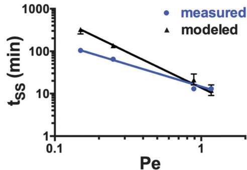
Fig. 6 Characteristic times of deposition ( t_{\text{SS}} ) as a function of Pe . t_{\text{SS}} is the time needed for \phi_{\text{electrode}} to reach 95% of its final value during deposition, as assessed from the results of Fig. 5. Blue data points are characteristic times for measurements, black data points are characteristic times for modeling. The curves are power laws: t_{\text{SS}}(Pe) = 13.5 \times Pe^{-1.091} for the measurements and, t_{\text{SS}}(Pe) = 16.2 \times Pe^{-1.568} for the model.
