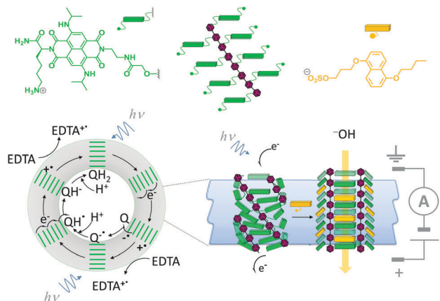
Fig. 16 A self-assembled synthetic transmembrane electron pump that can also open in response to ligand binding. 35 EDTA = ethylene diamine tetraacetate, Q = quinone.
