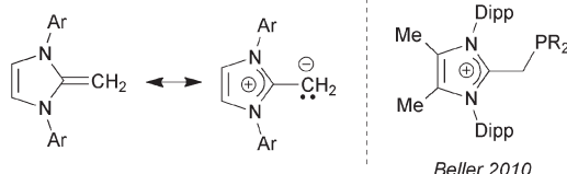
Chart 1 (Left) Canonical forms for a generic N-heterocyclic olefin (NHO); (Right) Beller's imidazolium alkylphosphines; \text{Ar} = \text{aryl} ; \text{Dipp} = 2,6\text{-}^i\text{Pr}_2\text{C}_6\text{H}_3 .
