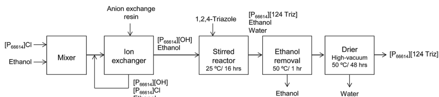
Fig. 2 Synthesis of [P_{66614}][124 \text{ Triz}] (adapted from Taylor et al. 7 ).
