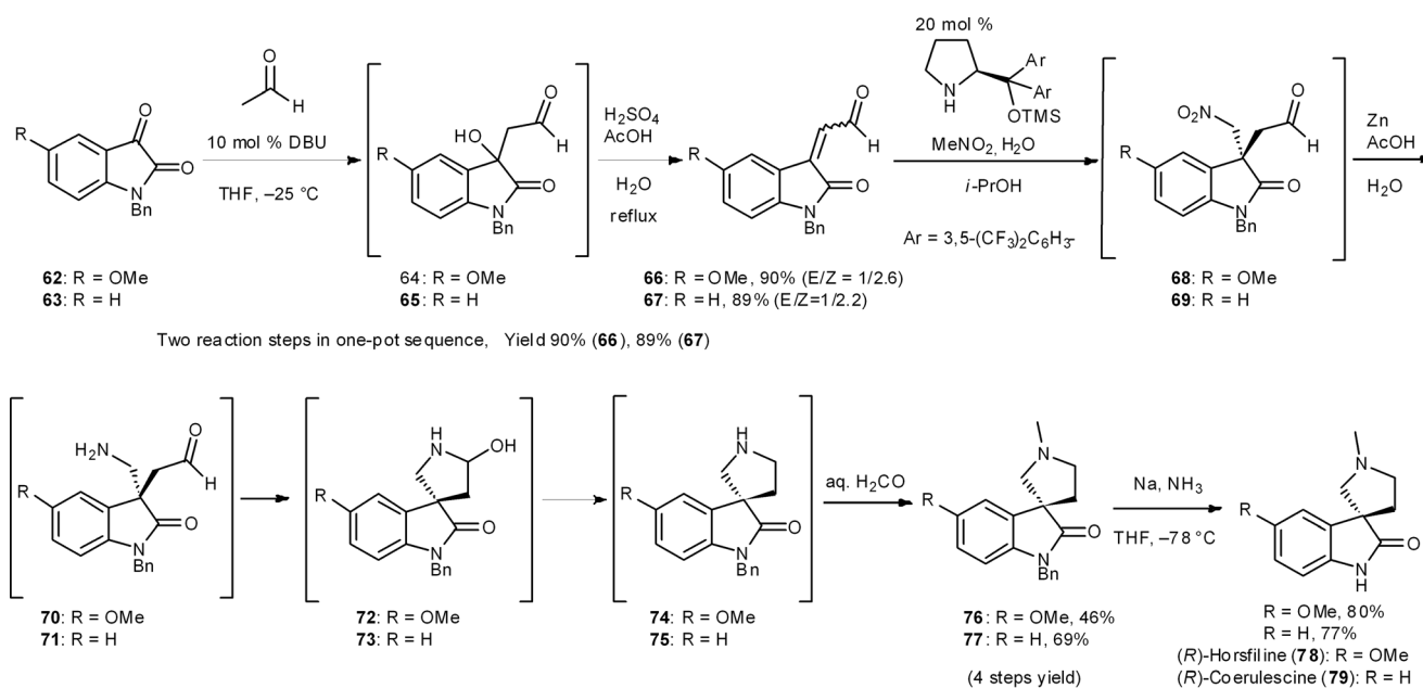
Scheme 7 Three-pot synthesis of (R)-horsfiline and (R)-coerulescine.
