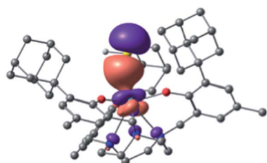
Fig. 6 Bonding \sigma orbital of [[((^{\text{Ad,Me}}\text{ArO})_3\text{tacn})\text{U}(\text{SH})] (2).
