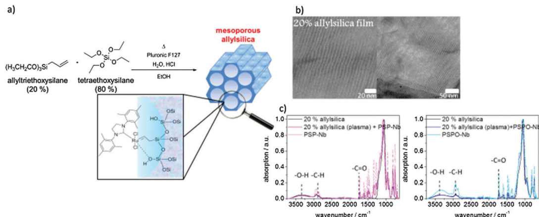
Fig. 6 (a) Schematic representation of the mesoporous allyltriethoxysilane containing silica mesoporous thin films and the binding of the ROP catalyst. (b) Representative TEM images of mesoporous silica thin films containing 20 mol% allyltriethoxysilane. (c) Infrared spectra for mesoporous allylsilica containing 20 mol% allyltriethoxysilane (black) and PSP- (pink) or PSPO-modified mesoporous allylsilica films (blue).
