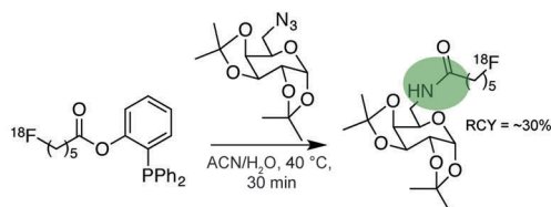
Fig. 41 (a) Click methods for radiosynthesis. (i) CuAAC click reaction for preparation of radiotracers including the synthesis of the most common prosthetic groups. (ii) 99m Tc(CO) 3 (H 2 O) 3 3+ radiolabelling through complexation by triazole moieties formed by CuAAC cycloaddition. (b) Copper-free click radiolabelling by SPAAC reaction. (i) 18 F introduced into the cyclooctyne prosthetic group ( 18 F-labelled aza-dibenzocyclooctyne derivative, [ 18 F]-ADIBO) and then subjected to strain-promoted cyclization with azide-functionalized biomolecules. 248 (ii) Labelling of ADIBO-functionalized biomolecules with 18 F-azides. 249 (c) Staudinger radiolabelling. 257 (d) Other examples of click radiolabelling. (i) Radiolabelling by oxime formation between an aminoxy-functionalized peptide and a 18 F-fluorobenzaldehyde ([ 18 F]FBA). (ii) Cyanobenzothiazole–cysteine (CBT–Cys) condensation reaction for 18 F-radiolabelling.
