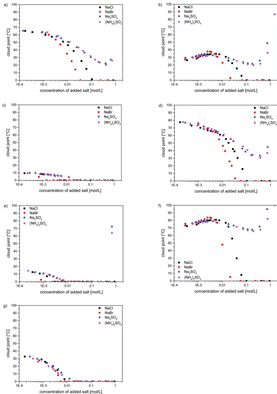
Fig. 5 Evolution of UCST-type cloud points of the polymer solutions in H 2 O (50 g L -1 ) containing inorganic salts for (a) P-1575, (b) P-395, (c) P-4585, (d) P-550, (e) P-6500, (f) P-785, and (g) P-8100. (■) = NaCl, (●) = NaBr, (▲) = Na 2 SO 4 , (▼) = (NH 4 ) 2 SO 4 .
