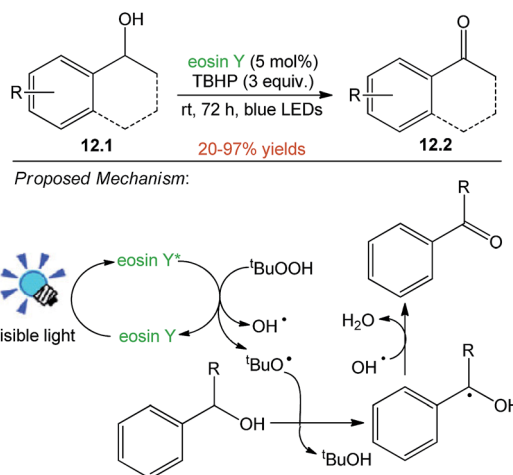
Scheme 12 Oxidation of benzyl alcohols.
