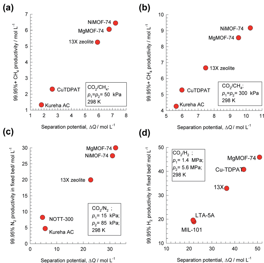
Fig. 6 Plots of the productivity of pure B, of specified purity, versus the separation potential, \Delta Q_{B/A} = Q_A \frac{y_B}{1-y_B} - Q_B , for A/B mixture separations in fixed beds. (a) 50/50 CO 2 /CH 4 mixture at 100 kPa, (b) 50/50 CO 2 /CH 4 mixture at 600 kPa, (c) 15/85 CO 2 /N 2 mixture at 100 kPa, and (d) 20/80 CO 2 /H 2 mixture at 7 MPa. All calculation details and structural information on the various MOFs are provided in the ESI.†
