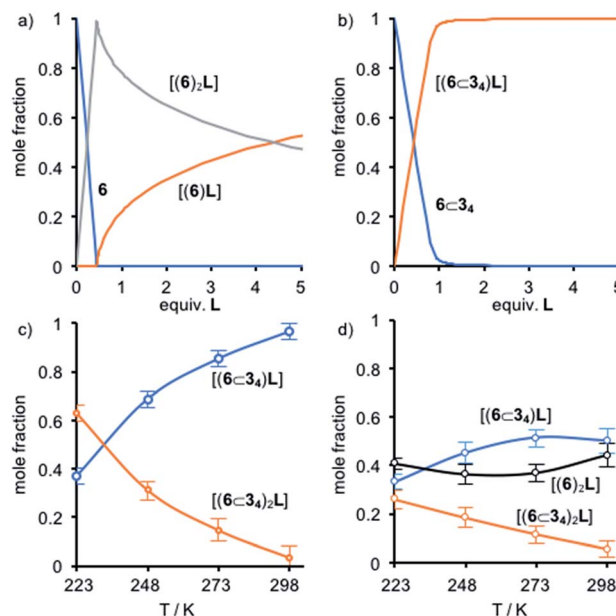
Fig. 4 Speciation diagrams for (a) 6 with respect to equiv. L ; (b) 6<3_4 with respect to equiv. L ; (c) L in a 6<3_4 + 0.4 L mixture with respect to T ; (d) L in a 6 + 6<3_4 + L (1 : 1 : 1) mixture with respect to T .
