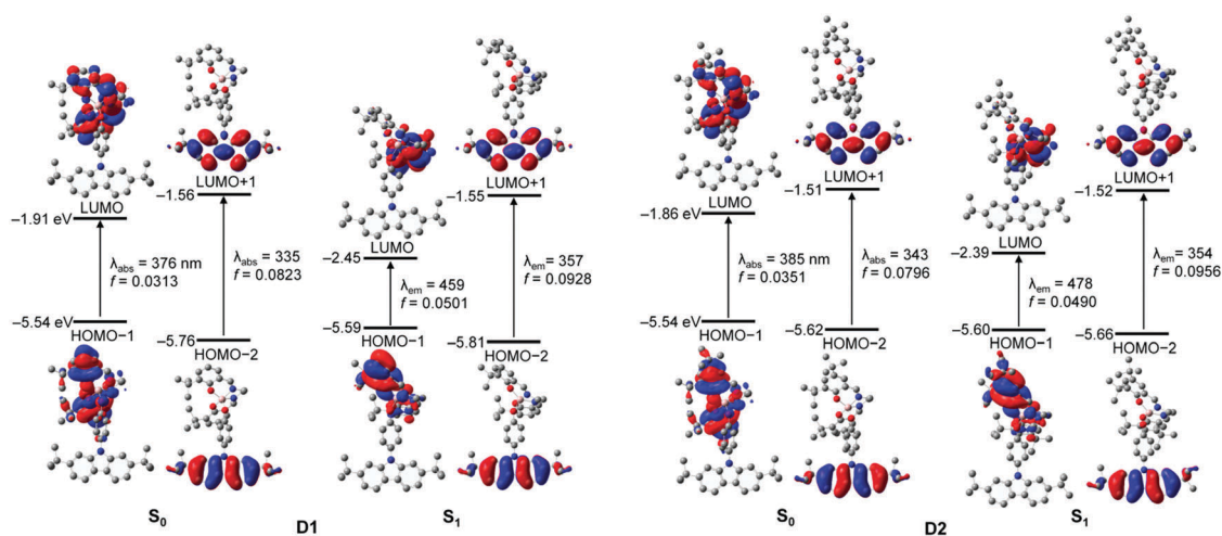
Fig. 5 Frontier molecular orbitals for D1 and D2 at their ground ( S_0 ) and first singlet ( S_1 ) state optimized geometries in THF and the major electronic transitions from TD-DFT calculations (isovalue = 0.04).
