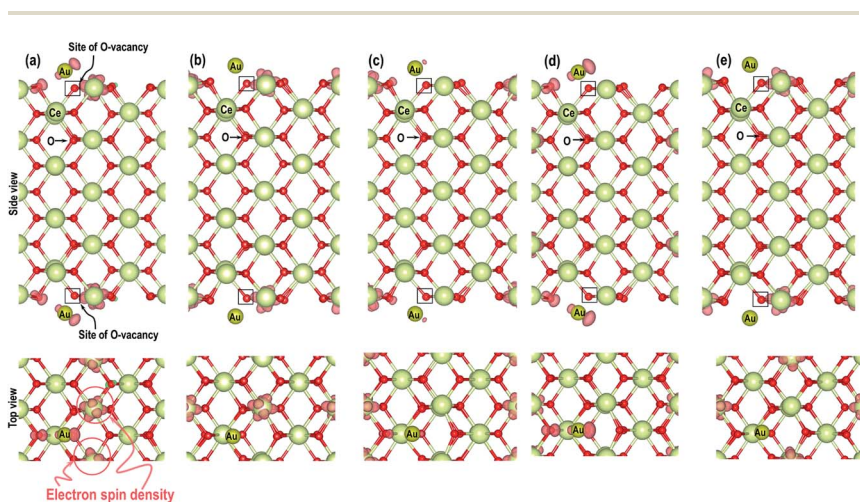
Fig. 6 Side and top views of electron spin density for the models (a) case 1, (b) case 2, (c) case 3, (d) case 4 and (e) case 5. The site of the O-vacancy is represented by an open black rectangular box and the pink lobe represents the electron spin densities with an isosurface of 0.007 e \text{\AA}^{-3} .
