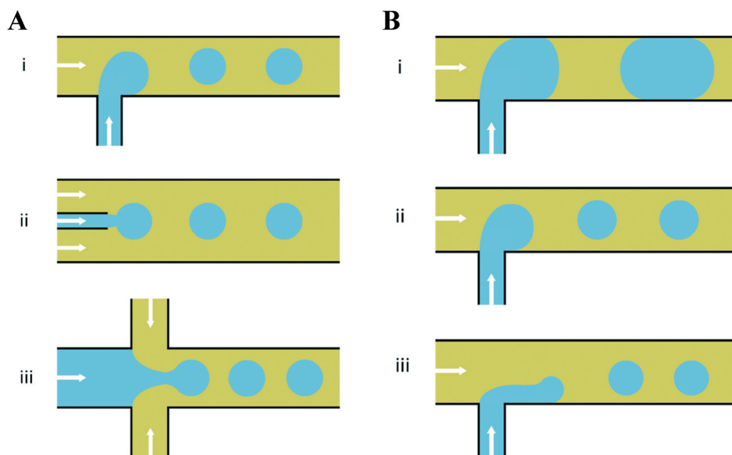
Fig. 2 Planar devices for droplet generation. (A) Microfluidic droplet generation geometries of (i) cross-flow, (ii) co-flow and (iii) flow-focusing. (B) Different modes of droplet break up in a microfluidic T-junction; (i) squeezing – droplets break up predominantly due to channel confinement at the microfluidic junction, yielding a ‘slug-like’ appearance (ii) dripping – as capillary number increases, viscous forces dominate over interfacial tension effects and droplet breakup occurs right at the dispersed nozzle and (iii) jetting – by increasing the continuous-fluid or dispersed-fluid flow rate, an extended liquid jet ultimately breaks up into droplets at the end of the jet. The arrows indicate the overall direction of bulk fluid flow and the blue and yellow colours indicate the dispersed and continuous phases, respectively.
