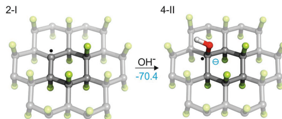
Fig. 9 Direct attack of a nucleophilic species (here \text{OH}^- ) on a radical site is energetically very favorable (energy in kcal mol ^{-1} in the gas phase).
