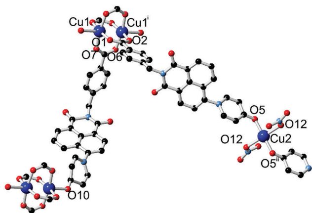
Fig. 6 (top) The two distinct copper coordination environments within the structure of 4 , with labelling scheme for coordinating heteroatoms. (bottom) Extended structure of a single layer of 4 , consisting of linear bridges between looped L2 -paddlewheel chains. Hydrogen atoms and backbone disorder are omitted for clarity. Symmetry codes used to generate equivalent atoms: (i) 1/2 - x, 3/2 - y, 1 - z ; (ii) 2 - x, 1 - y, 2 - z .
