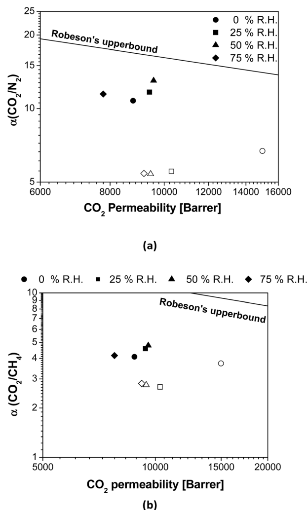
Fig. 3 Comparison of (a) \text{CO}_2/\text{N}_2 and (b) \text{CO}_2/\text{CH}_4 selectivity as a function of R.H. with the Robeson's upper bound. 9 Open symbols: PTMSP. Filled symbols: zeolite A/PTMSP MMM. The symbols indicate the direction towards increasing relative humidity values as follows: 0% (circles) < 25% (squares) < 50% (triangles) < 75% (rhombuses).
