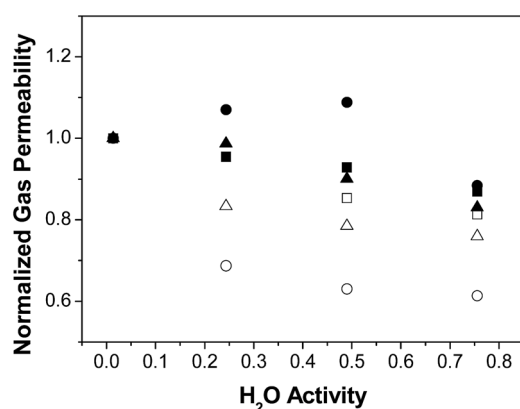
Fig. 2 Normalised gas permeability P/P_{\text{dry}} through the zeolite A/PTMSP MMM, (full symbols) PTMSP membranes (void symbols): \text{N}_2 (triangles), \text{CH}_4 (squares), \text{CO}_2 (circles).
