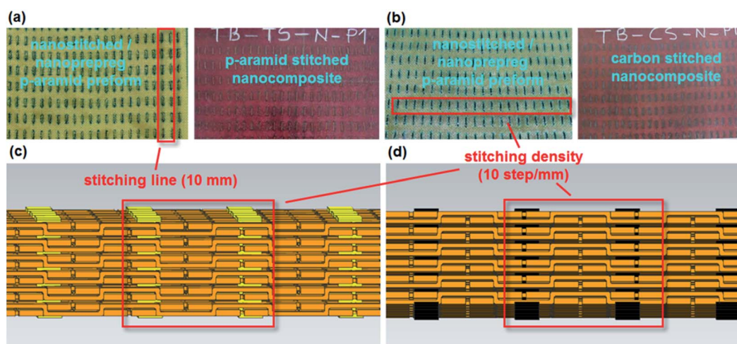
Fig. 2 (a) Para-aramid Twaron CT multistitched 3D nanoprepreg preform (left) and p-aramid/phenolic MWCNT composite (right) (TB-TS-N); (b) PAN carbon multistitched 3D nanoprepreg preform (left) and p-aramid/phenolic MWCNT composite (right) (TB-CS-N); (c) schematic view of p-aramid stitched p-aramid structure (TB-TS); (d) schematic view of carbon stitched p-aramid structure (TB-CS).
