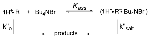
Scheme 3 Associative mechanism involving the fast and reversible formation of a reactive 1 : 1 adduct between the added salt and the ion pair \text{1H}^+ \cdot \text{R}^- . The latter corresponds to \text{B}'' in Scheme 1.
