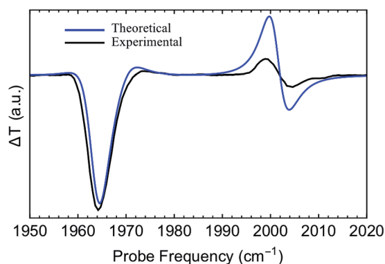
Fig. 9 Experimental and theoretical pump-probe (differential) transmission spectra of strongly coupled \text{W}(\text{CO})_6 in an optical microcavity. 57 These results correspond to the case where the cavity photon and the molecular vibration (asymmetric C=O stretch) are resonant.
