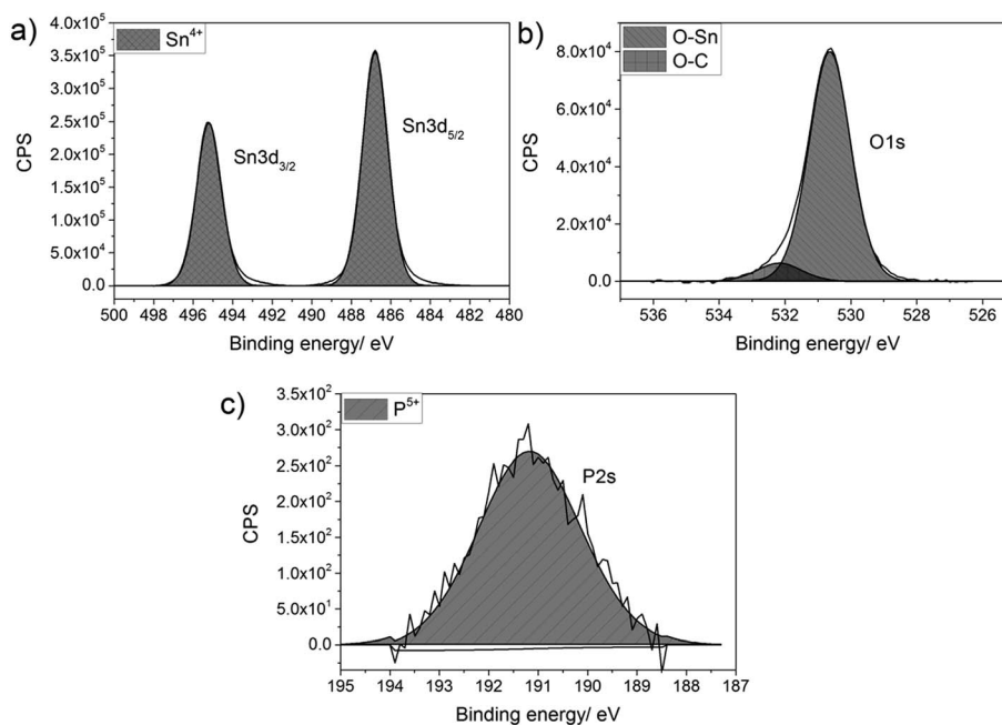
Fig. 1 Typical X-ray photoelectron spectra for (a) Sn 3d environment, (b) O 1s environment and (c) P 2s environment for P-doped SnO 2 films synthesised by AACVD at 550 \text{ }^\circ\text{C} .
